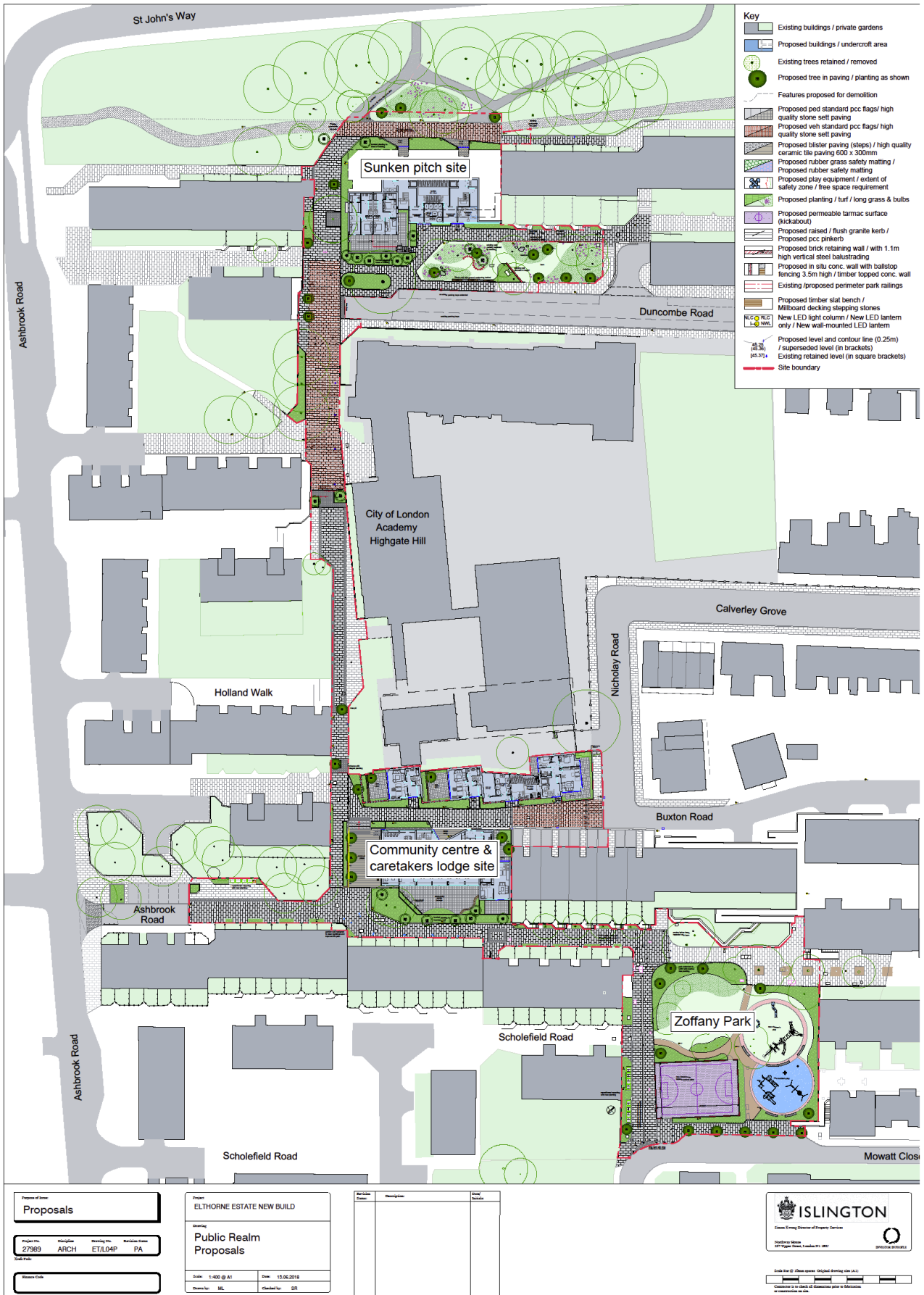
Figure 1: Elthorne Estate Sunken Pitch & CC Master Site-plan incl landscaping/public realm
